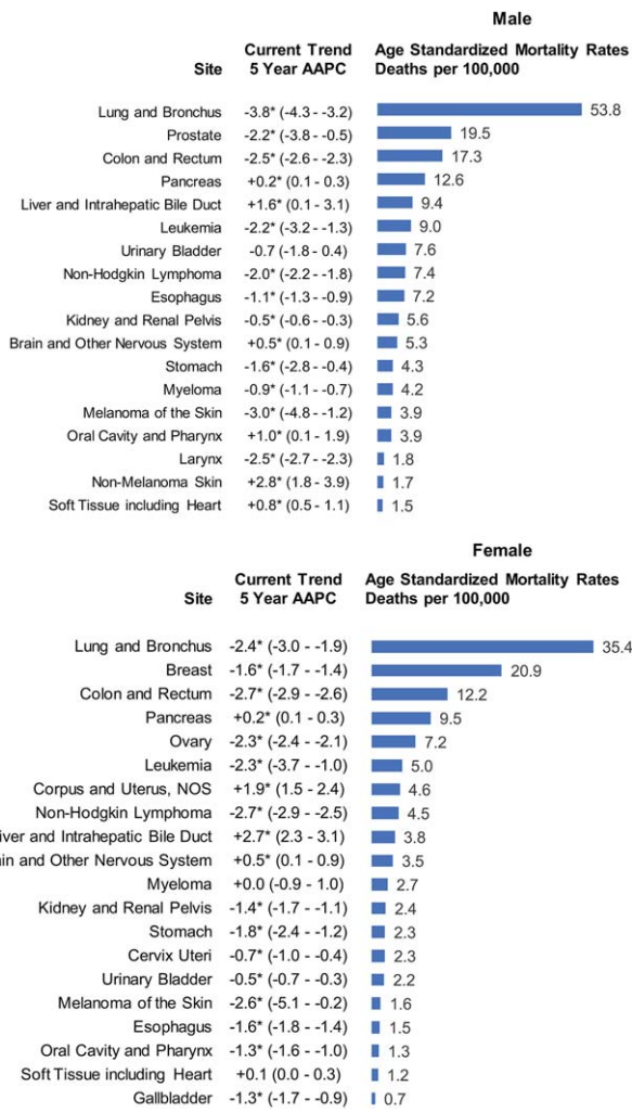
Figure 3. Age-standardized death rates and recent fixed-interval trends (2011-2015) are illustrated for the 18 most common cancers in men and the 20 most common cancers in women, for all races/ethnicities combined, and by sex. The 5-year average annual percent change (AAPC) is based on the joinpoint trend from 1999 to 2015. An asterisk indicates that the AAPC is statistically significantly different from zero (2-sided t test or Z test; P < .05). Rates were age-standardized to the 2000 US standard population (19 age groups; Bureau of the Census. Current Population Reports, Publication 25-1130. Washington, DC: US Government Printing Office; 2000 [Census P25-1130]). The AAPC is a weighted average of the annual percent changes over the fixed interval (2011-2015) using the underlying joinpoint model for the period from 1999 to 2015. Joinpoint models with up to 3 joinpoints are based on rates per 100,000 persons age standardized to the 2000 US standard population (19 age groups; Census P25-1130). For joinpoint analysis, the Joinpoint Regression Program was used (version 4.5.0.1; Bethesda, MD: Statistical Research and Applications Branch, National Cancer Institute; June 2017).
